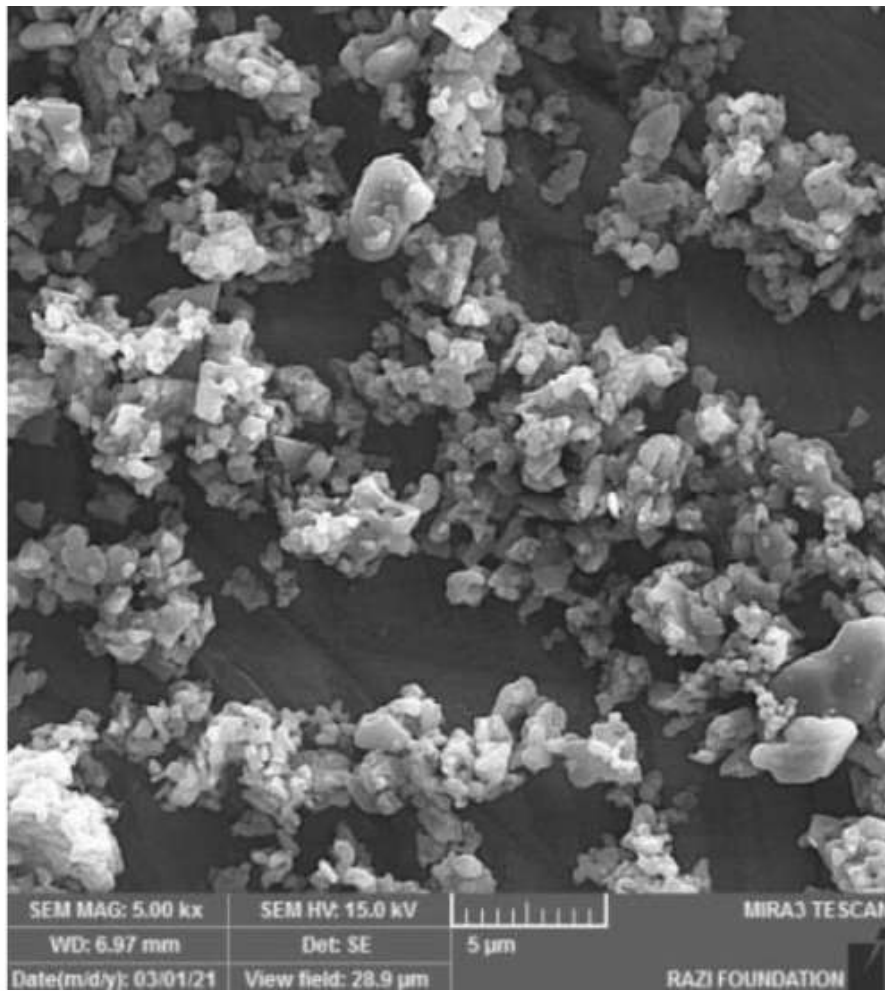
SEM image of Al 2 O 3 powder.
