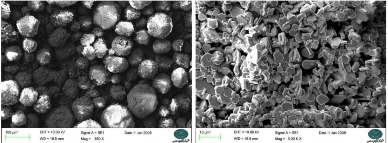
SEM image of Al 2 O 3 powder.
